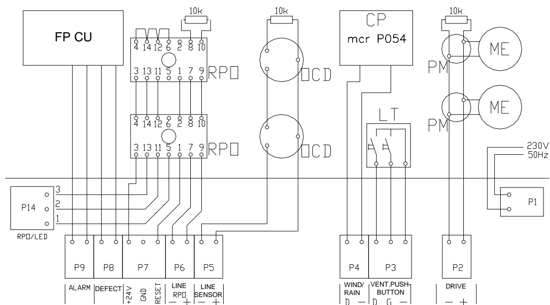
Fig. 3 Typical configuration of smoke exhaust system with mcr 0204 unit.
